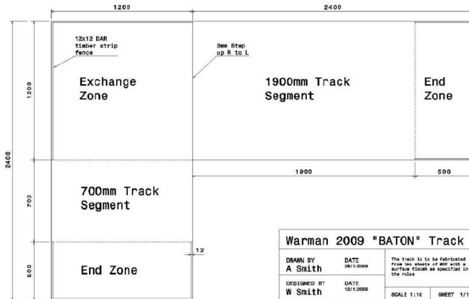
FIGURE 2 - PROJECT "BATON" COMPETITION TRACK (Plan View)
